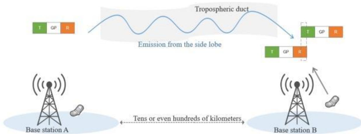
The proportion of the propagation delay goes beyond the guard period
