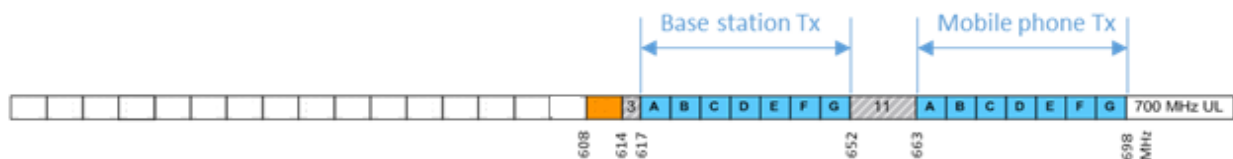
Frequency arrangement from US incentive auction
