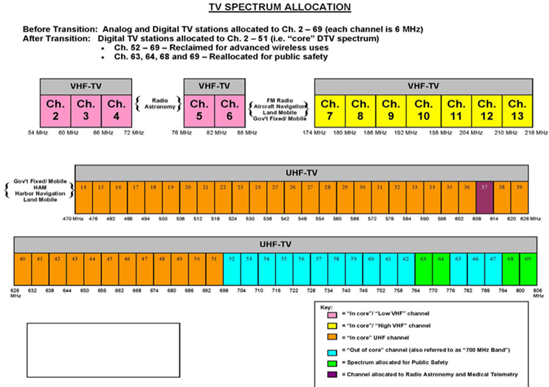
FIGURE 10 TV allocation in the United States of America
